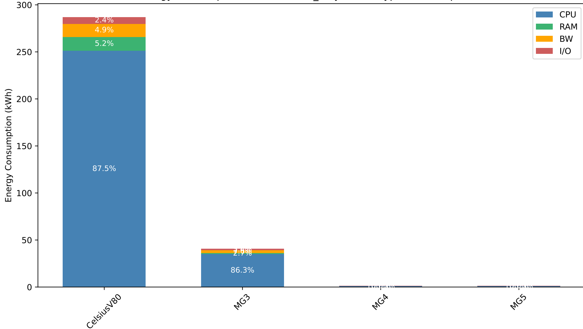
Energy Consumption in Datacenter_1 by Server Type and Component
